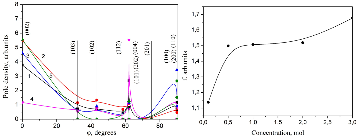
Figure 3. Pole density P_i , and orientation factor f_i , as a function of the incidence angle \phi between the direction and the normal to the reflection plane for films obtained at different concentrations of thiourea (1 - 0.1 M, 2 - 0.5 M, 3 - 1 M, 4 - 2 M, 5 - 3 M)
